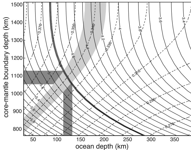
Figure 3. Ocean and core-mantle boundary depths for one physical structure: 20 km ice shell, cold thermal structure, pyrolytic mantle, and iron core composition. Solid lines contour mass (in 10^{22} Kg); dashed lines are for moment of inertia values. Uncertainties in the two discontinuity depths, denoted by dark gray boxes, are due to uncertainties in mass, equal to 4.800 \pm 0.015 \times 10^{22} kg (thick contour line), and uncertainties in moment of inertia ( 0.346 \pm 0.005 [ Anderson et al., 1998 ]), denoted by light gray.
